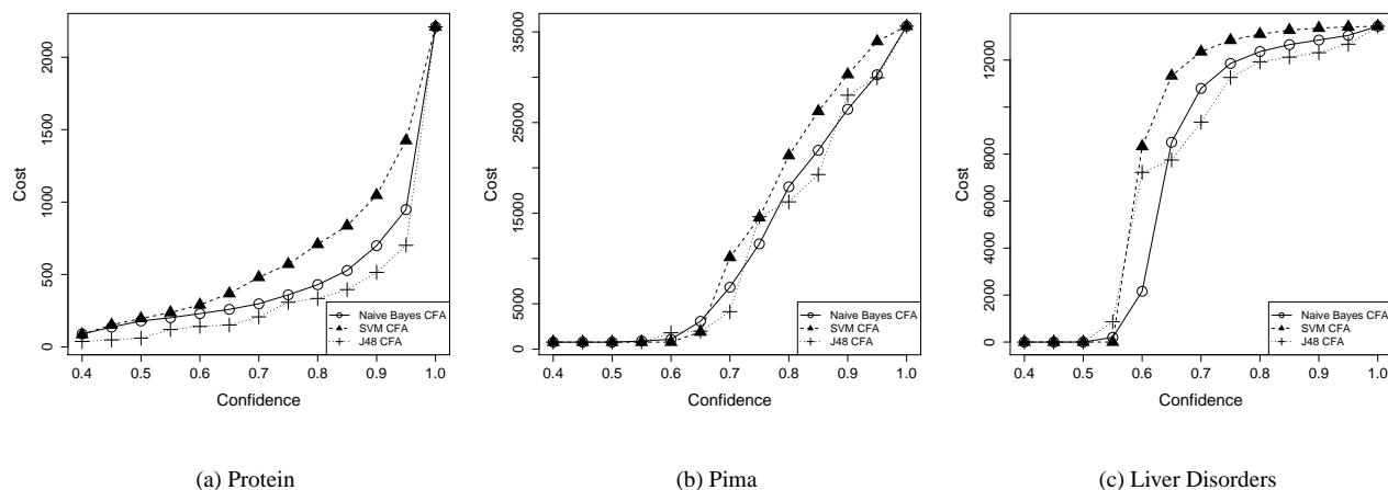
Figure 8: Total feature acquisition cost results for CFA using different base classifiers.
